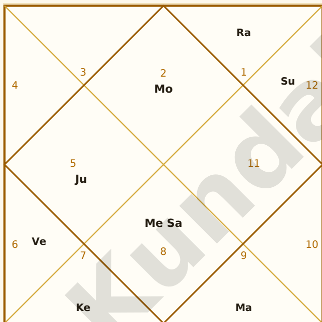
Navamsa (D9)
