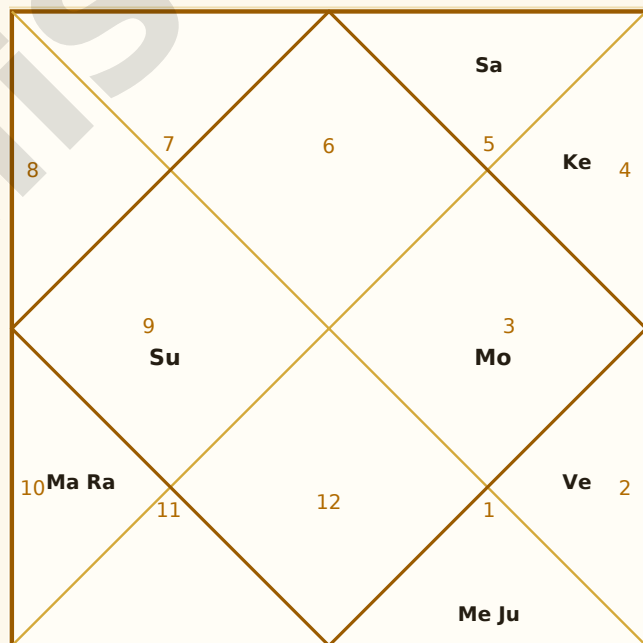
Dasamsa (D10)
